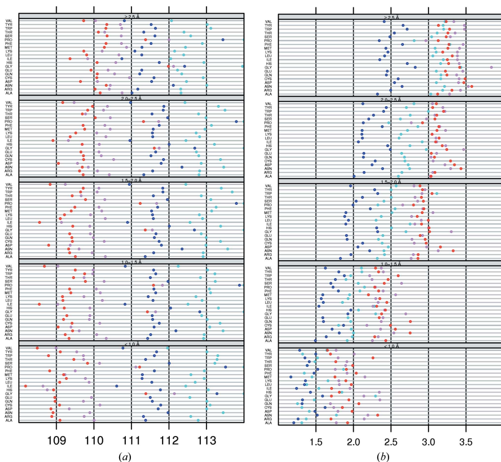
Figure 7 The average \tau (a) and standard deviation on \tau (b) for residues in a helix ('H', dark blue), in a strand ('S', red), in a loop with \varphi , \psi angles in the helix area ('C_A', light blue) and in a loop with \varphi , \psi angles in the strand area ('C_B', pink). Dark blue and red circles are the same as in Figs. 1 and 4. We chose to use the same x-axis range as in the other figures for clarity. Gly and Pro \tau angles that are higher than 114^\circ are shown at 114^\circ . The true values are available from the associated web pages.
